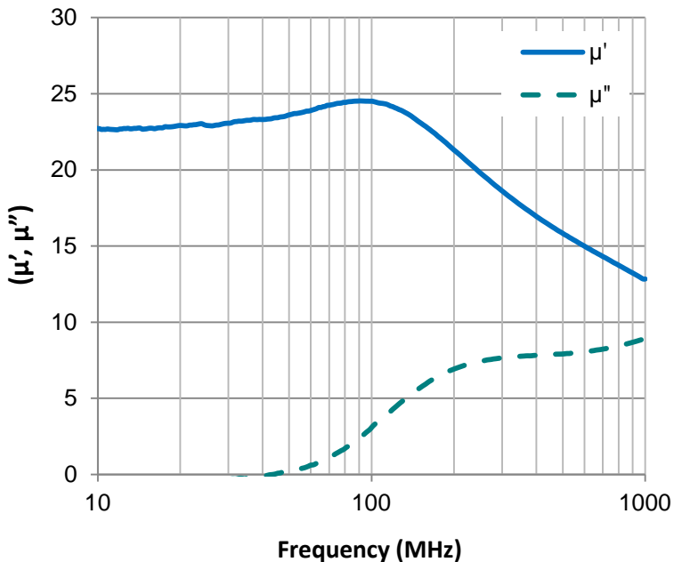
Measured Complex Permeability
