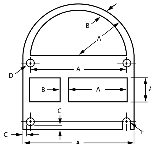
Figure 1 DIE-CUT GASKET
