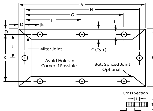
Figure 2 SPLICED GASKET
