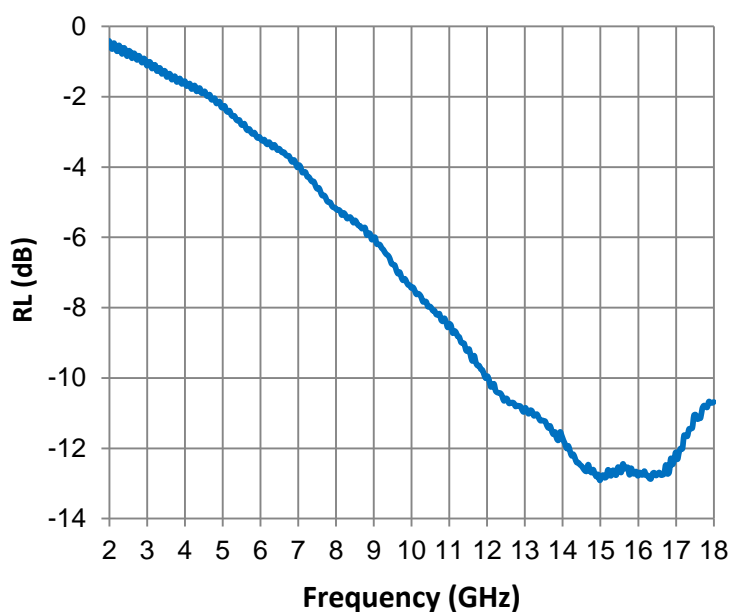
Reflection Loss
