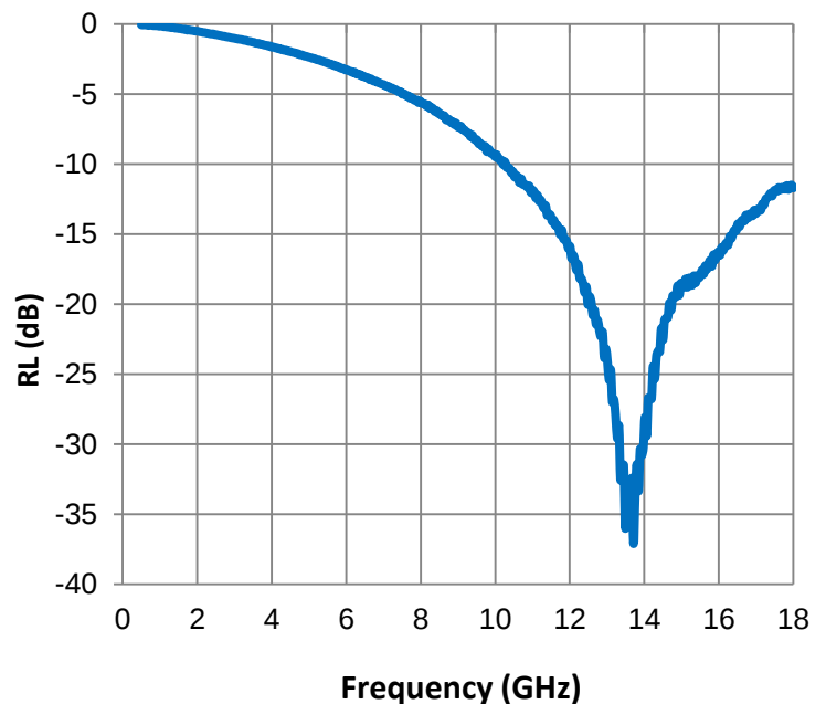
Reflection Loss
