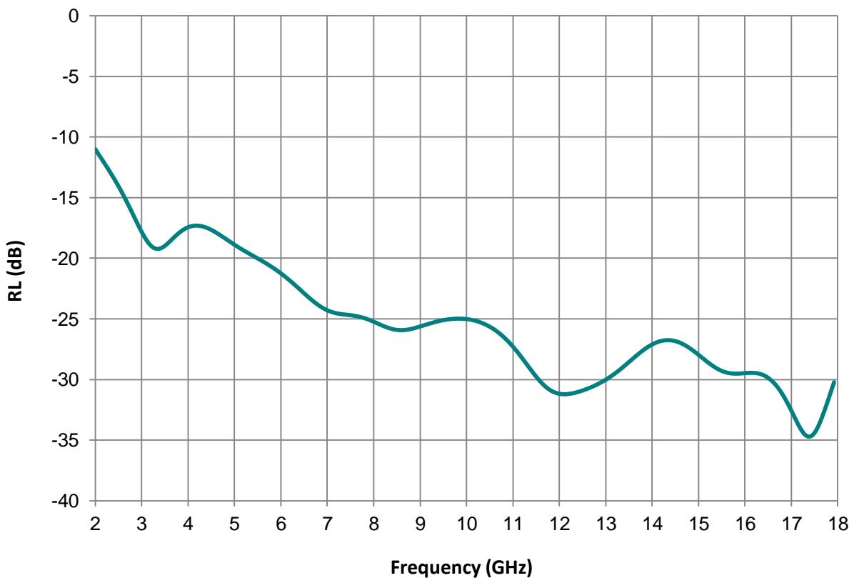
Reflection Loss of RT-10003
