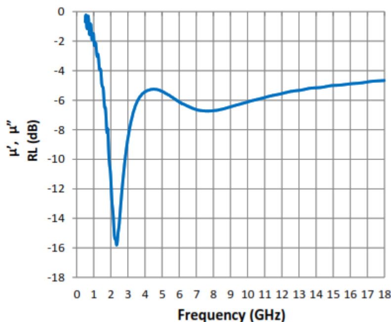
Reflection Loss
