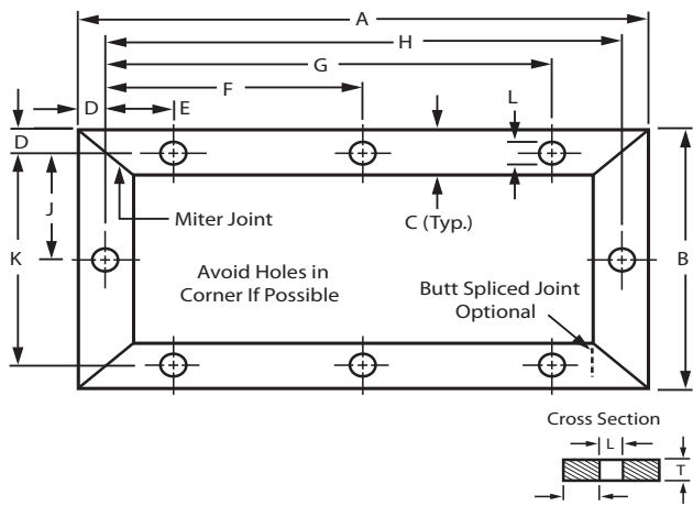
Figure 2 SPLICED GASKET
