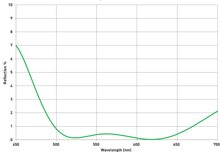
Reflectance of 4 ohm/sq ITO Glass Index Matched to Air
